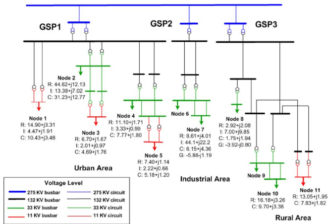
Fig. 1. Reference network comprising rural, urban, and industrial areas.
