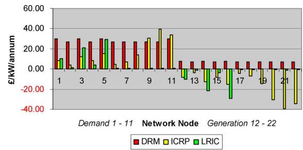
Fig. 2. Marginal costs derived from each pricing model.
