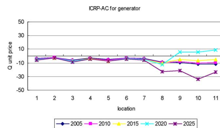
Fig. 9. ICRP-AC generation reactive power price evolution.
