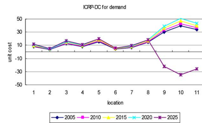
Fig. 6. Nodal price evolution for demand with ICRP model.
