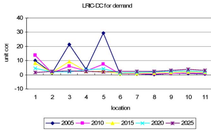
Fig. 10. Nodal price evolution for demand with LRIC model.
