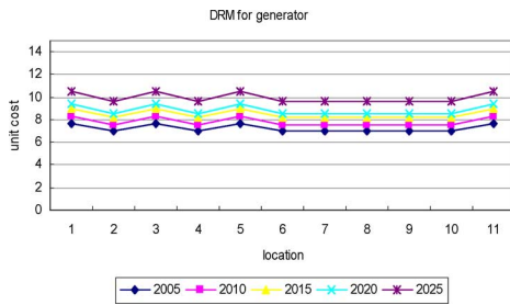
Fig. 5. Nodal prices evolution for generation with DRM model.
