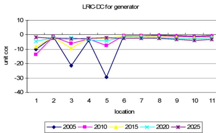
Fig. 11. Nodal price evolution for generation with LRIC model.
