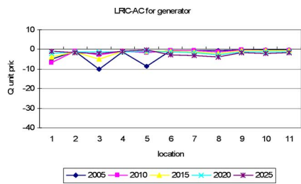
Fig. 13. LRIC generation real power price evolution.
