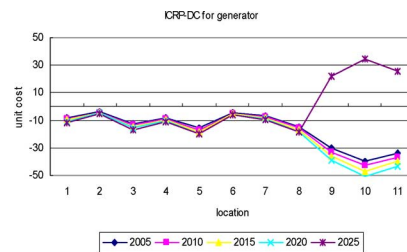
Fig. 7. Nodal price evolution for generation with ICRP model.
