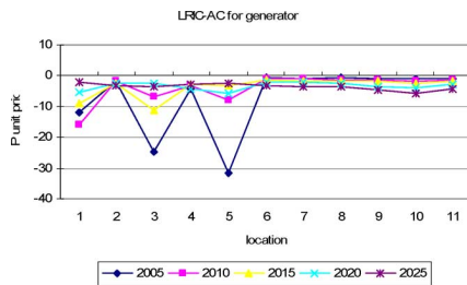
Fig. 12. Nodal price evolution for LRIC model.
