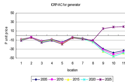
Fig. 8. ICRP-AC generation real power price evolution.
