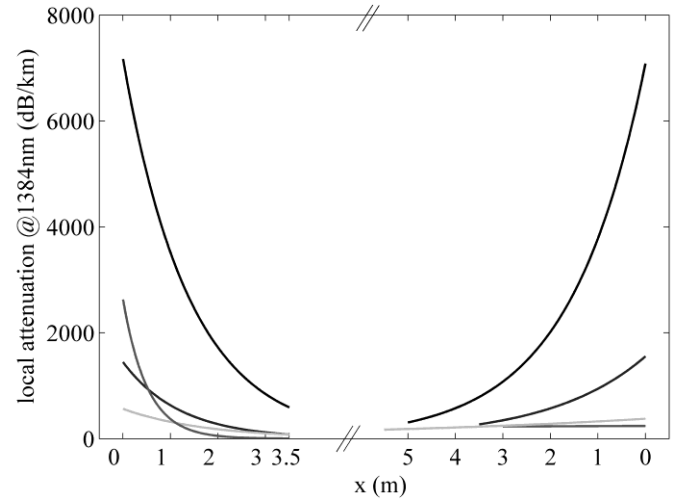
Fig. 9. Local attenuation for all fibers at 1384 nm, x is the length from the end to the center of the fibers. From black to light gray 1.3 \mu\text{m} , 2.5 \mu\text{m} , 5.2 \mu\text{m} core diameter and HC-PCF (fibers A, B, C and D).
