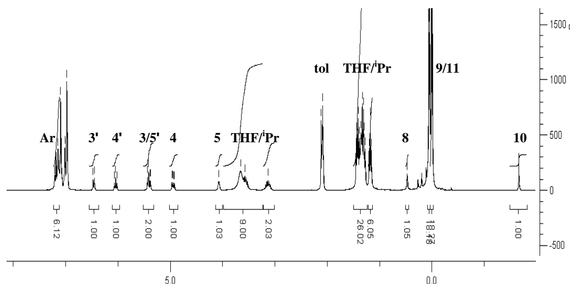
Figure 2. Annotated ^1H NMR spectrum of the dearomatized calcium complex 4 .
