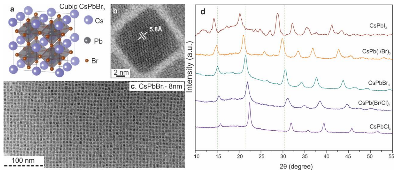
Figure 1. Monodisperse CsPbX 3 NCs and their structural characterization. (a) Schematic of the cubic perovskite lattice; (b,c) typical transmission electron microscopy (TEM) images of CsPbBr 3 NCs; (d) X-ray diffraction patterns for typical ternary and mixed-halide NCs.
