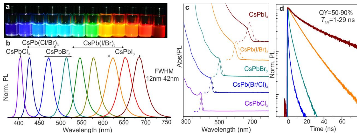
Figure 2. Colloidal perovskite \text{CsPbX}_3 NCs ( X=\text{Cl}, \text{Br}, \text{I} ) exhibit size- and composition-tunable bandgap energies covering the entire visible spectral region, with narrow and bright emission: (a) colloidal solutions in toluene, under UV lamp ( \lambda=365 nm); (b) representative PL spectra ( \lambda_{\text{exc}}=400 nm for all, but 350 nm for \text{CsPbCl}_3 samples); (c) typical optical absorption and PL spectra; (d) time-resolved PL decays for all samples shown in (c), except \text{CsPbCl}_3 .
