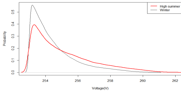
Figure 4 Probability distribution of over voltage in high summer and winter
