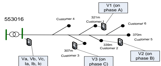
Figure 2 Sample of data Acquisition
